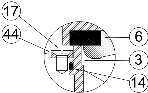
ONE PIECE SEAT &amp; BOTTOM GUIDE DETAILS
