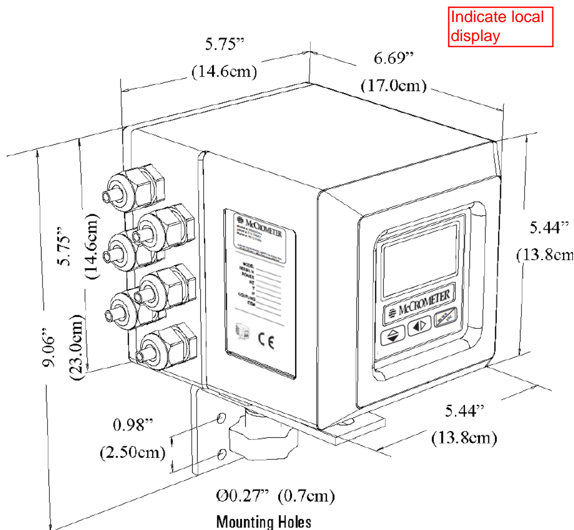
Figure 13: Local Converter Dimensions
