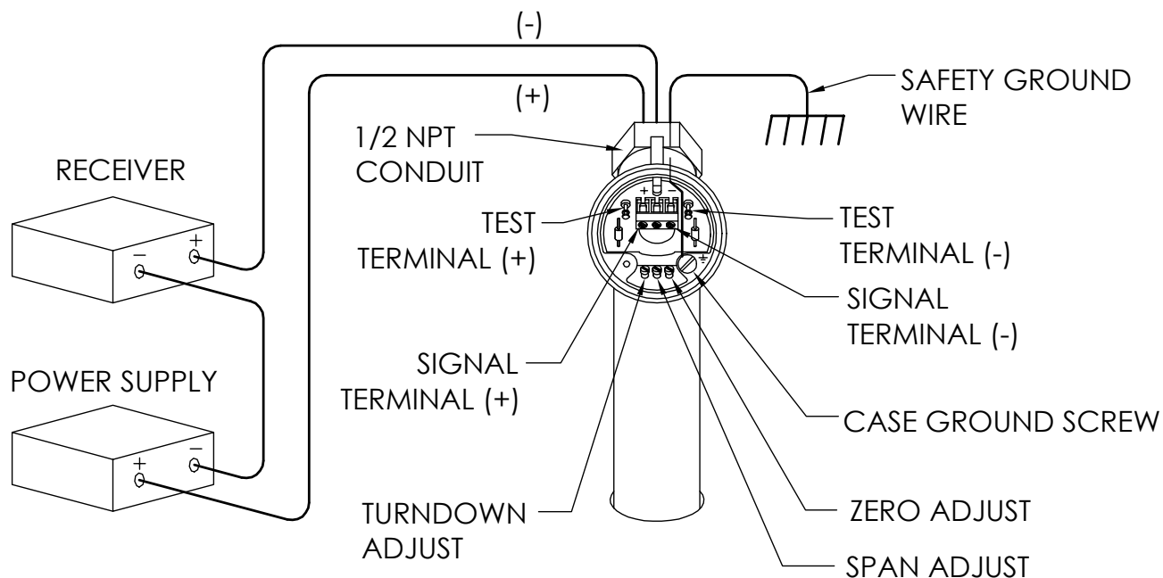
FIGURE 2-3 MODEL 88F WIRING
