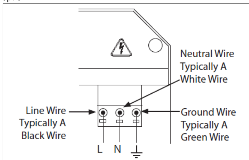
Figure 22: AC Power Wiring
