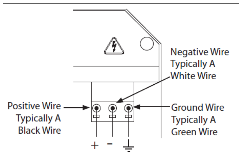
Figure 23: DC Power Wiring
