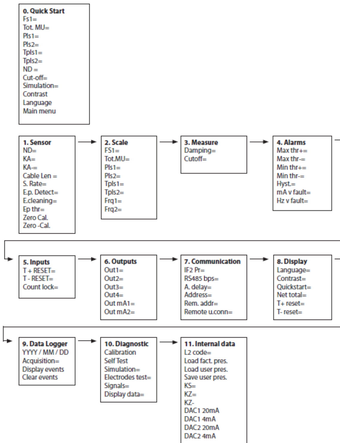
Figure 30: Menu Structure
