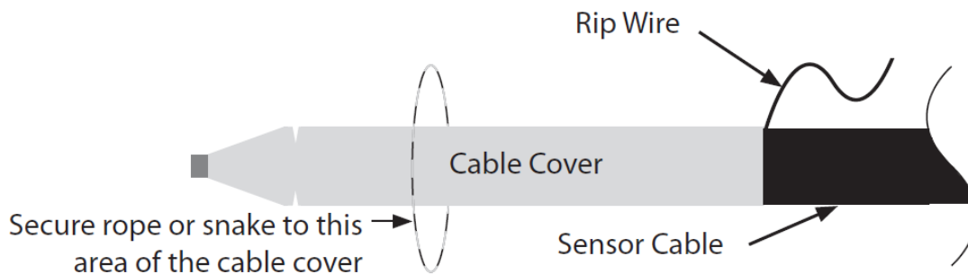
Figure 16: Cable Cover
