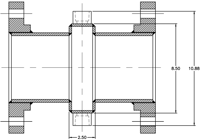
SECTION X-X
