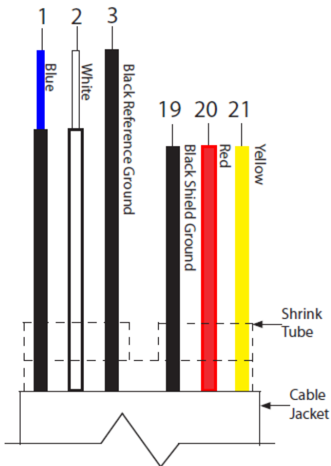
Figure 18: Wire Labeling
