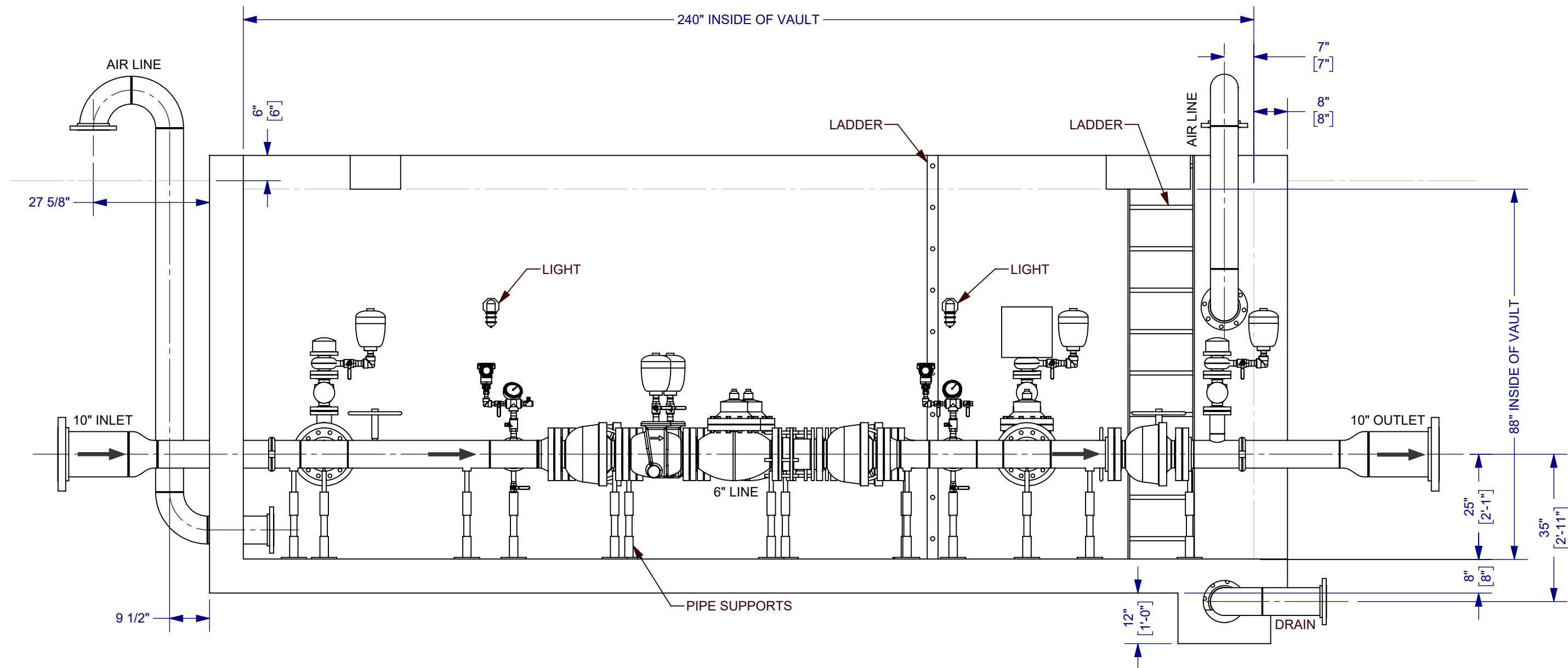
ELEVATION VIEW
