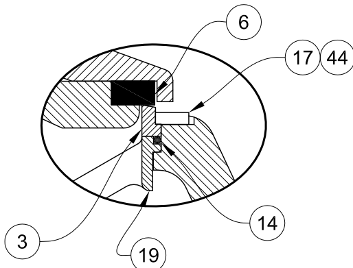
TWO PIECE SEAT &amp; BOTTOM GUIDE DETAILS
