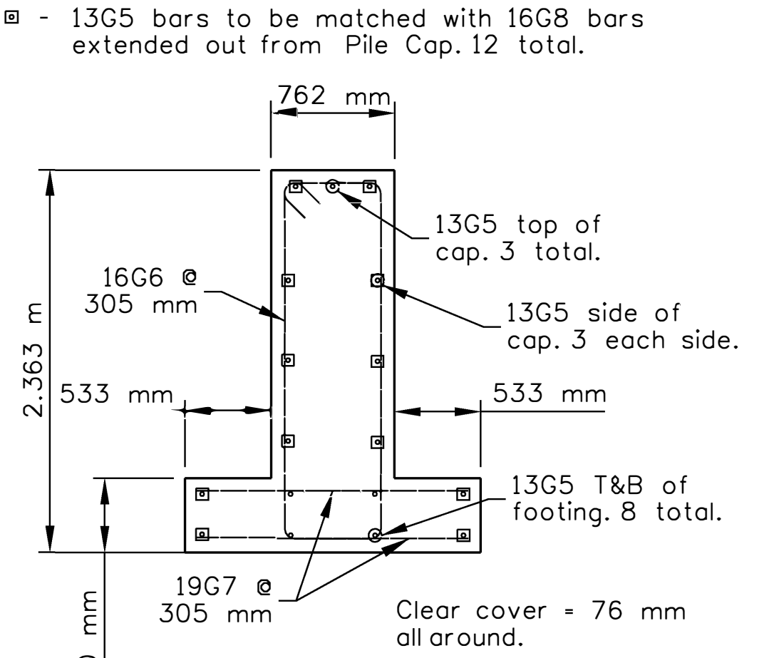
SECTION B-B (THROUGH WINGWALL FOOTING)
