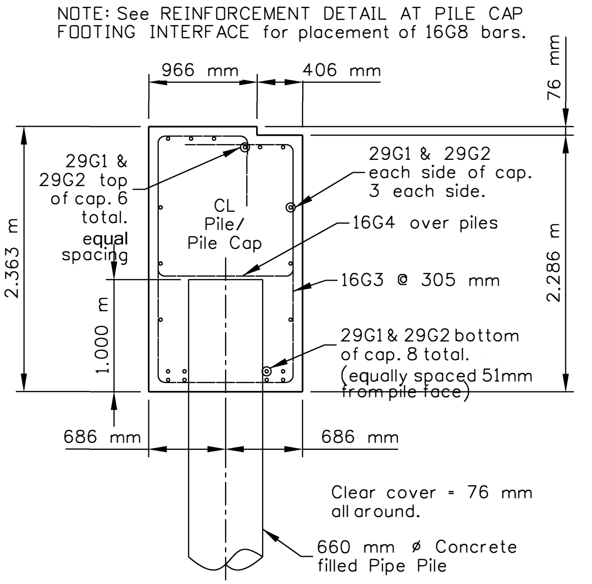
SECTION A-A (THROUGH PILE CAP)
