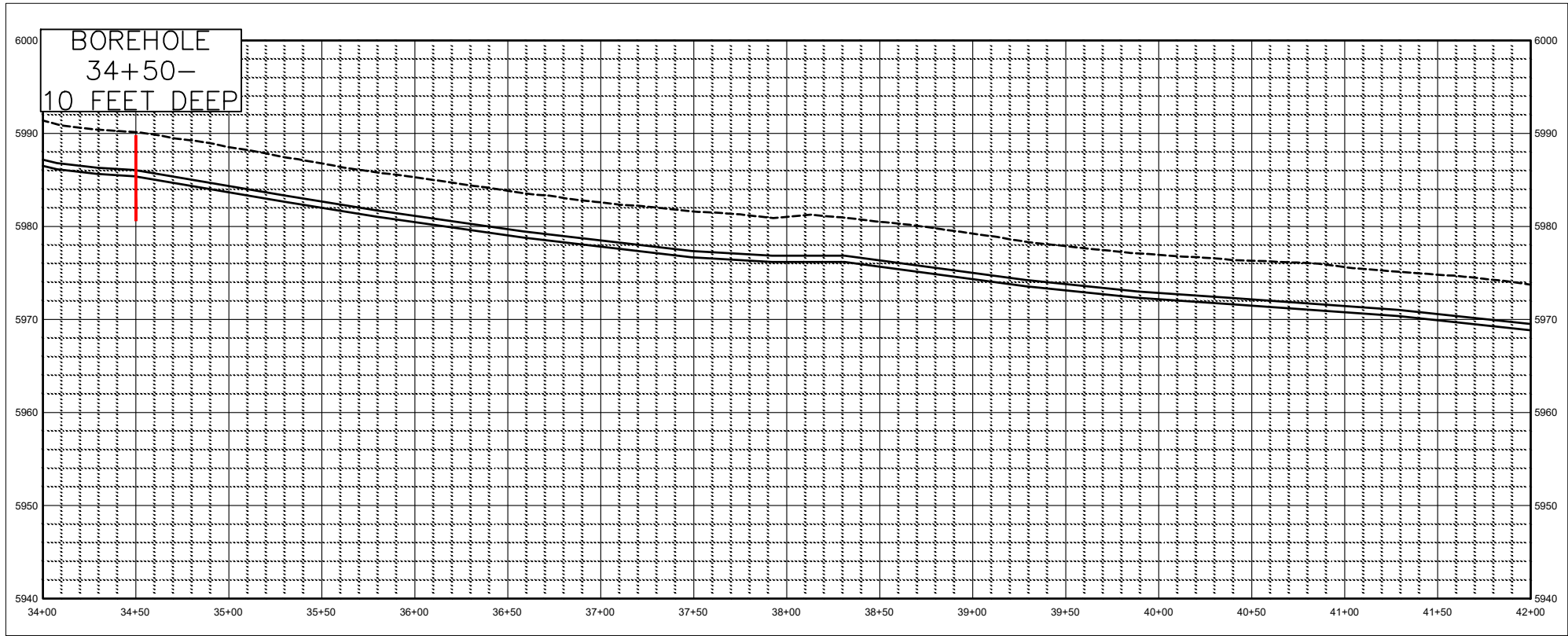
PROFILE SCALE = 1"=40'
