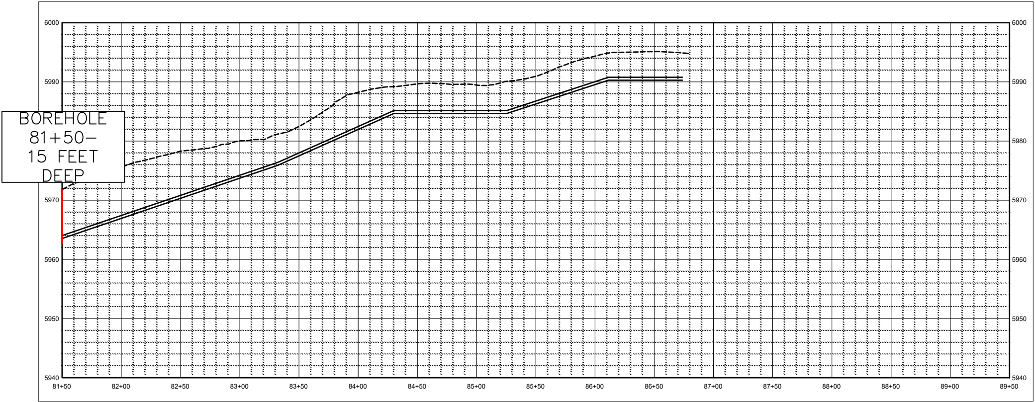
PROFILE
