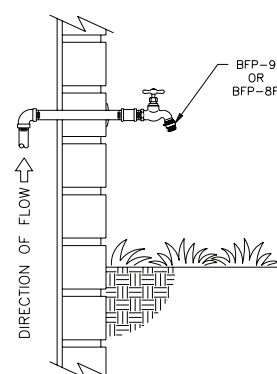
TYPICAL HOSE BIBB INSTALLATION
